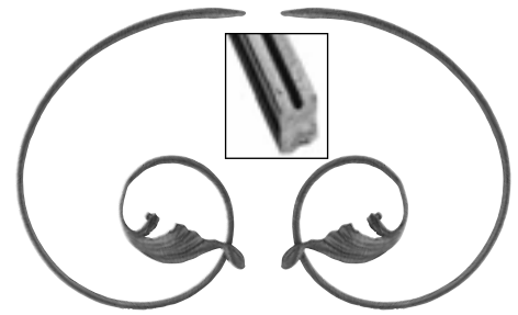
Art. 682/9 Ø 16 x 8 mm H 330 mm L 230 mm
