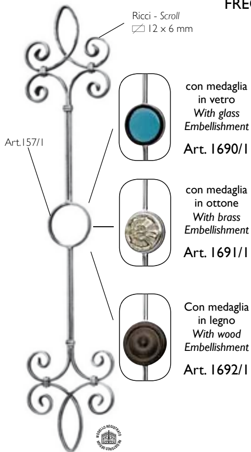
Art. 1688/5 \square 12 x 12 mm H 1000 mm L 200 mm
