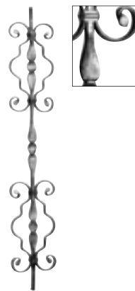
Art. 134/D/1 ∅ 12 x 6 mm H 900 mm Art. 134/D/2 ∅ 12 x 12 mm H 900 mm Art. 134/D/3 ∅ 12 x 12 mm H 1200 mm
