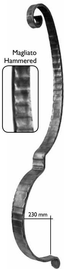
Art. 109/2 □ 60 x 8 mm H 1000 mm
