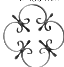
Art. 454/5 12 x 6 mm Ø 300 mm
