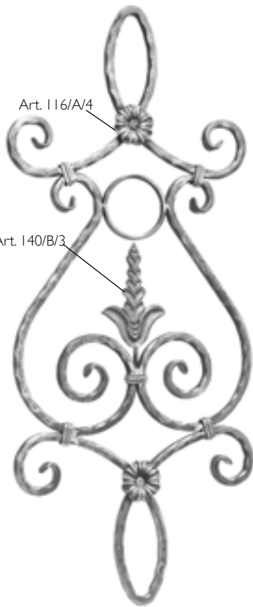
Art. 475/2 \Phi 12 x 12 mm H 900 mm L 380 mm spigolato hammered on edges
