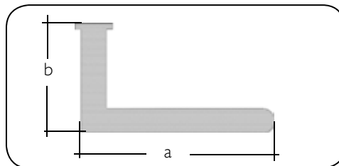
Art. 1476/1 a = 129 - b = 100 mm (coppia - couple)
