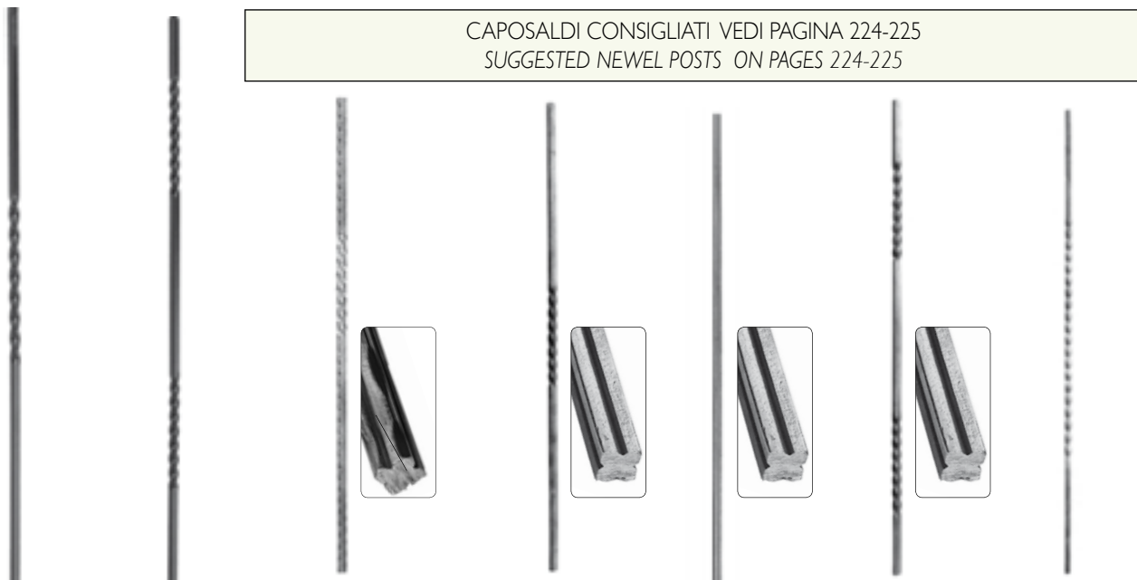
Art. 1160/7 \Phi 12 x 12 mm H 1200 mm Art. 1160/8 \Phi 12 x 12 mm H 1200 mm Art. 639/5 \Phi 20 x 20 mm H 1200 mm Art. 639/6 \Phi 12 x 12 mm H 900 mm Art. 118/H/2 \Phi 12 x 12 mm H 900 mm Art. 118/H/30 \Phi 12 x 12 mm H 1000 mm Art. GD35/4 \Phi 12 x 12 mm H 1000 mm Art. 118/H/1 \Phi 12 x 12 mm H 900 mm Art. 118/H/29 \Phi 12 x 12 mm H 1000 mm Art. 55/3 \Phi 8 x 8 mm H 820 mm Art. 55/4 \Phi 8 x 8 mm H 900 mm
