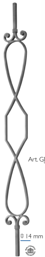
Art. GDI78/1 Ø 14 x 8 mm H 1000 mm L 120 mm
