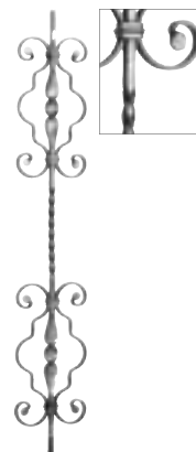
Art. 134/C/4 ∅ 12 x 6 mm H 900 mm Art. 134/C/5 ∅ 12 x 12 mm H 900 mm Art. 134/C/6 ∅ 12 x 12 mm H 1200 mm
