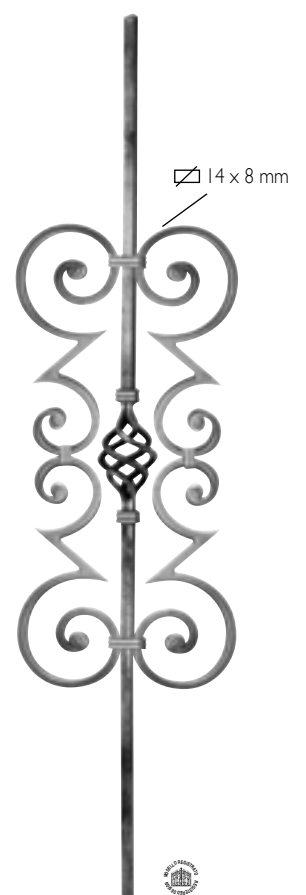
Art. GD200/3 \Phi 14 x 14 mm H 1000 mm L 215 mm
