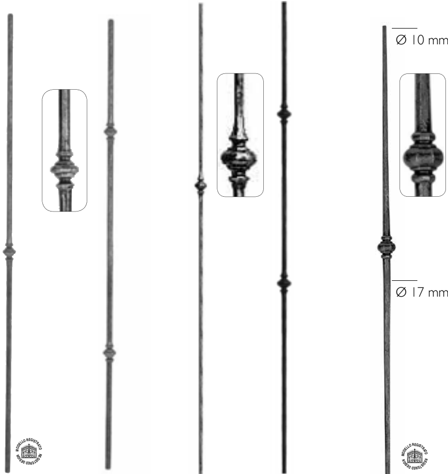
Art. 1770/2 Art. 1771/2 Art. 1159/1 Art. 1159/2 Art. 1184/5 Ø 12 mm Ø 12 mm Ø 12 mm Ø 12 mm Ø 10 mm H 1000 mm H 1000 mm H 1200 mm H 1200 mm Ø 17 mm Conico/Conic
