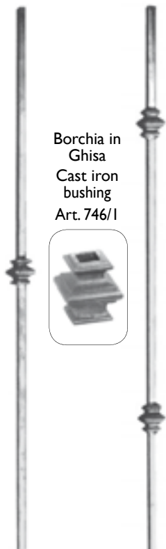
Art. 755/5 Art. 755/6 Φ 12 x 12 mm Φ 12 x 12 mm H 900 mm H 900 mm
