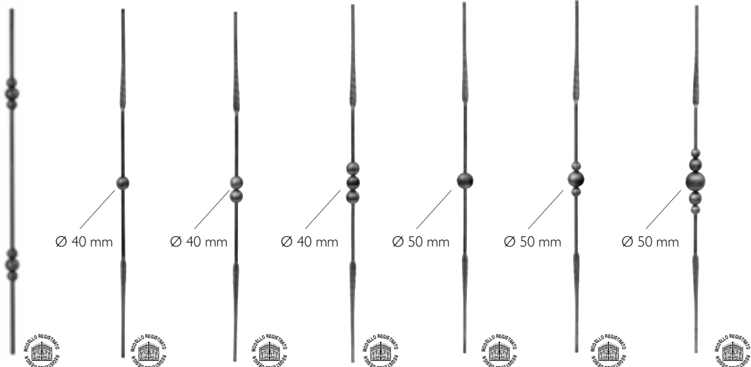
Art. GD48/1 Art. I210/1 Art. I210/2 Art. I210/3 Art. I210/4 Art. I210/5 Art. I210/6 Ø 12 mm Ø 12 mm Ø 12 mm Ø 12 mm Ø 12 mm Ø 12 mm Ø 12 mm H 1000 mm H 1000 mm H 1000 mm H 1000 mm H 1000 mm H 1000 mm H 1000 mm
