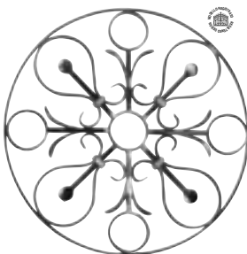
Art. 1024/1 □ 12 x 6 mm Ø 615 mm
