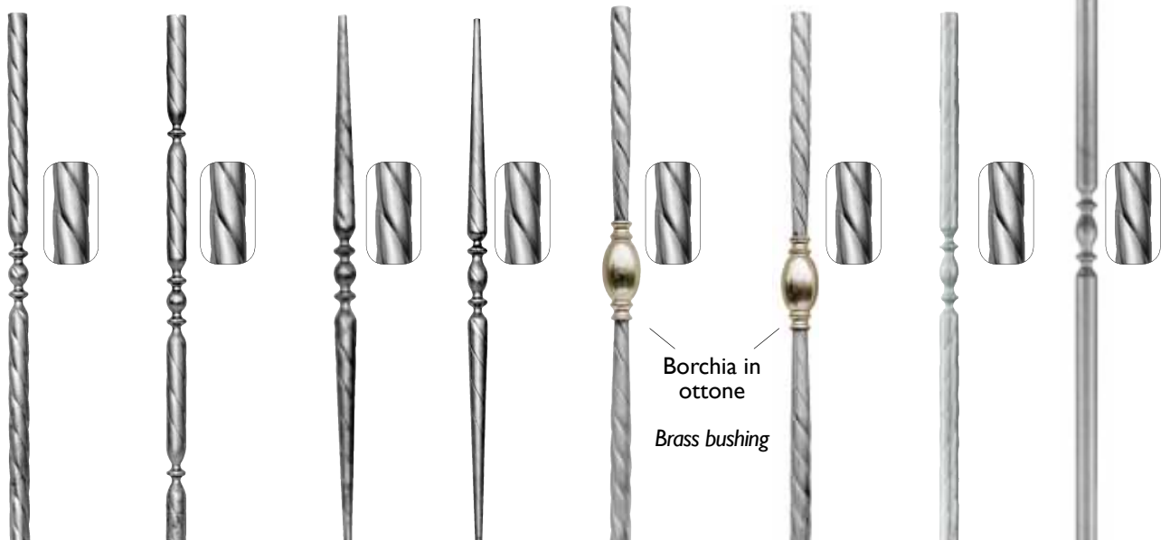
Art. I794/1 Art. I794/2 Art. I794/3 Art. I794/4 Art. I794/5 Art. I794/6 Art. I794/7 Art. I794/8 Ø 40 mm Ø 40 mm Ø 40 mm Ø 40 mm Ø 40 mm Ø 40 mm Ø 40 mm Ø 40 mm H 1000 mm H 1000 mm H 1000 mm H 1000 mm H 1000 mm H 1000 mm H 1000 mm H 1200 mm
