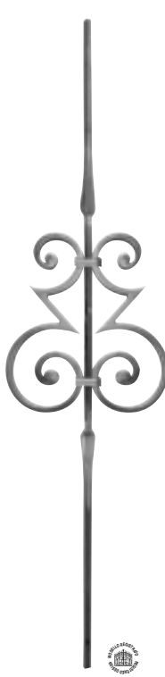
Art. GDI99/3 Φ 14 x 14 mm H 1000 mm L 215 mm
