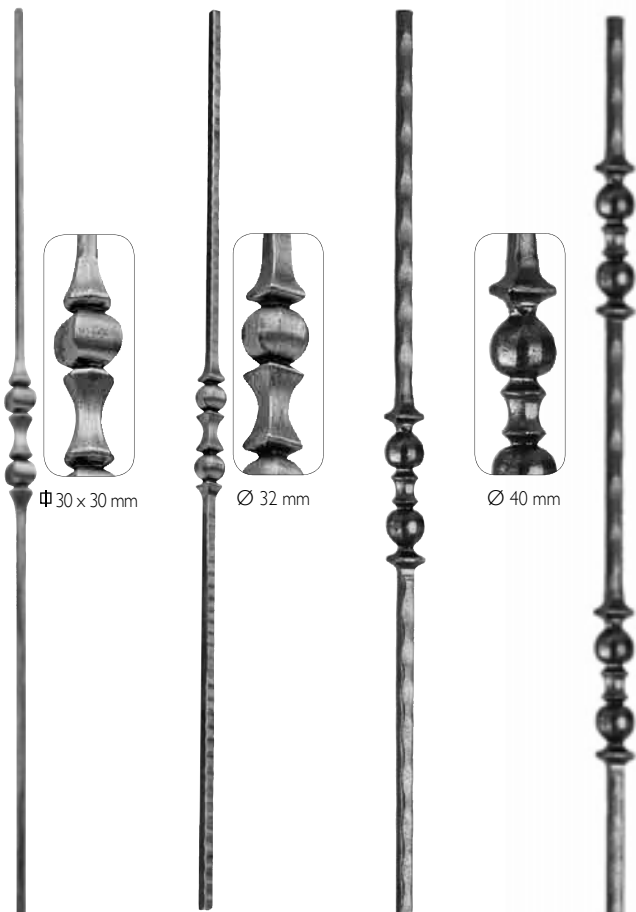
Art. 1769/3 Ø 12 mm H 1000 mm Art. 1769/4 Φ 12 x 12 mm H 1000 mm Art. 1770/5 Φ 14 x 14 mm H 1000 mm Art. 1771/5 Φ 14 x 14 mm H 1000 mm
