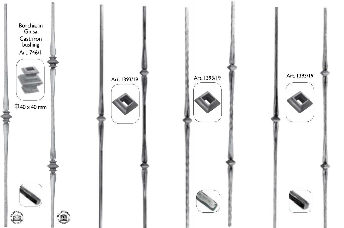
Art. 1176/3 Art. 1176/4 Art. 1746/1 Art. 1746/2 Art. 1746/3 Art. 1746/4 Art. 1746/5 Art. 1746/6 Ø 12 mm Ø 12 mm Ø 12 mm Ø 12 mm Ø 12 mm Ø 12 mm Ø 12 mm Ø 12 mm H 1000 mm H 1000 mm H 1000 mm H 1000 mm H 1000 mm H 1000 mm H 1000 mm H 1000 mm
