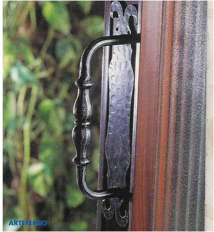
Art. 839/2 H 200 mm Ø 25 mm Rosetta/Rosette Ø 60 mm
