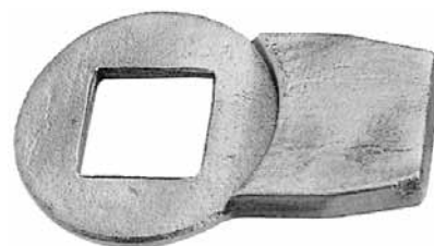
Art. 609/1 Ø 70 mm 30 ÷ 40 x 8 mm Foro/Hole Φ 30 x 30 mm
