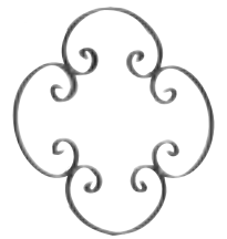
Art. 24/C/2 □ 10 x 5 mm Ø 380 mm
