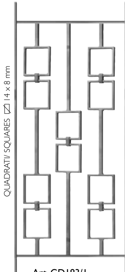
Art. GDI83/1 \square 14 x 8 mm H 1000 mm L 400 mm
