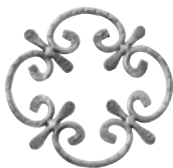
Ø 260 mm Art. 26/1 Ø 10 mm Art. 26/2 Ø 8 mm
