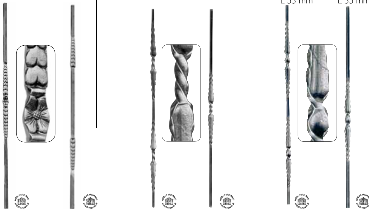
Art. 1718/13 Φ 12 × 12 mm H 1000 mm Art. 1718/15 Φ 12 × 12 mm H 1000 mm Art. 1730/1 Φ 12 × 12 mm H 1000 mm Art. 1730/3 Φ 12 × 12 mm H 1000 mm Art. 1730/5 Φ 12 × 12 mm H 1000 mm Art. 1730/7 Φ 12 × 12 mm H 1000 mm Art. 1718/14 Φ 14 × 14 mm H 1000 mm Art. 1718/16 Φ 14 × 14 mm H 1000 mm Art. 1730/2 Φ 14 × 14 mm H 1000 mm Art. 1730/4 Φ 14 × 14 mm H 1000 mm Art. 1730/6 Φ 14 × 14 mm H 1000 mm Art. 1730/8 Φ 14 × 14 mm H 1000 mm
