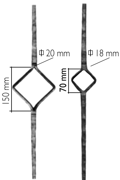
Art. 108/2 Art. 108/1 H 1000 mm H 1000 mm
