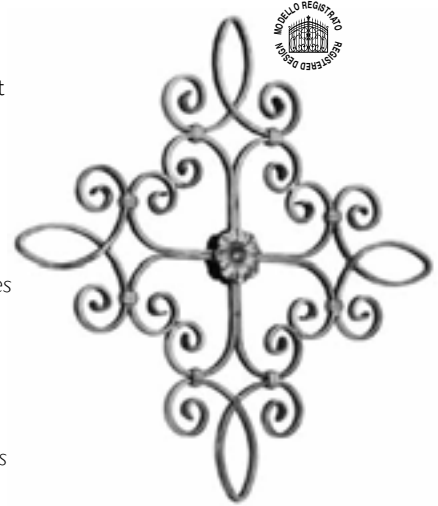
Art. 1647/I 12 x 6 mm H 610 mm L 440 mm
