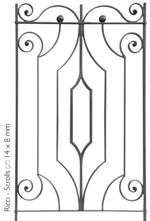
Art. GD242/I \Phi 12 x 12 mm H 1000 mm - L 640 mm
