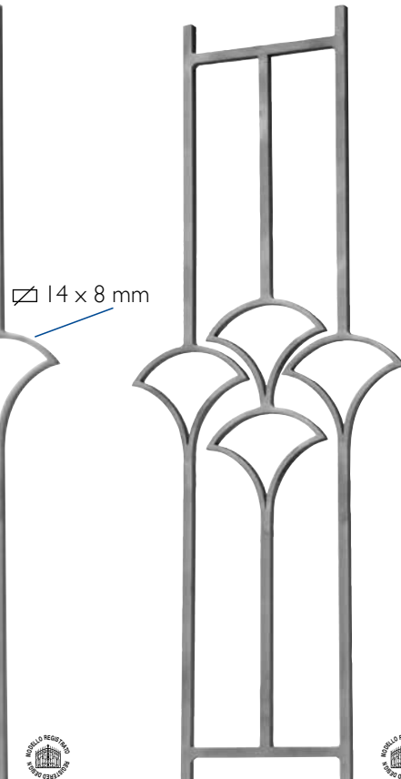
Art. GDI86/2 \Phi 14 x 14 mm H 1000 mm L 390 mm
