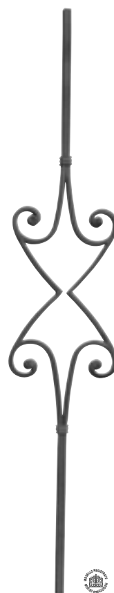
Art. GDI54/1 \Phi 14 x 14 mm H 1000 mm L 190 mm
