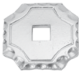
Art. 1448/6 70 x 70 mm foro/hole 12 x 12 mm spess./thick. 4 mm
