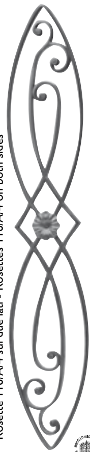
Art. 1681/1 □ 14 x 8 mm H 1000 mm L 190 mm
