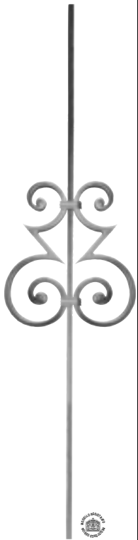
Art. GDI99/1 □ 14 x 8 mm H 1000 mm L 210 mm
