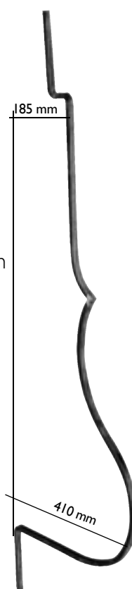
Φ 14 x 14 mm Art. 1271/5 H 1200 mm Art. 1271/6 H 1400 mm Art. 1271/7 H 1600 mm Art. 1271/8 H 1800 mm
