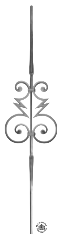
Art. GDI95/6 Φ 14 x 14 mm H 1000 mm L 215 mm
