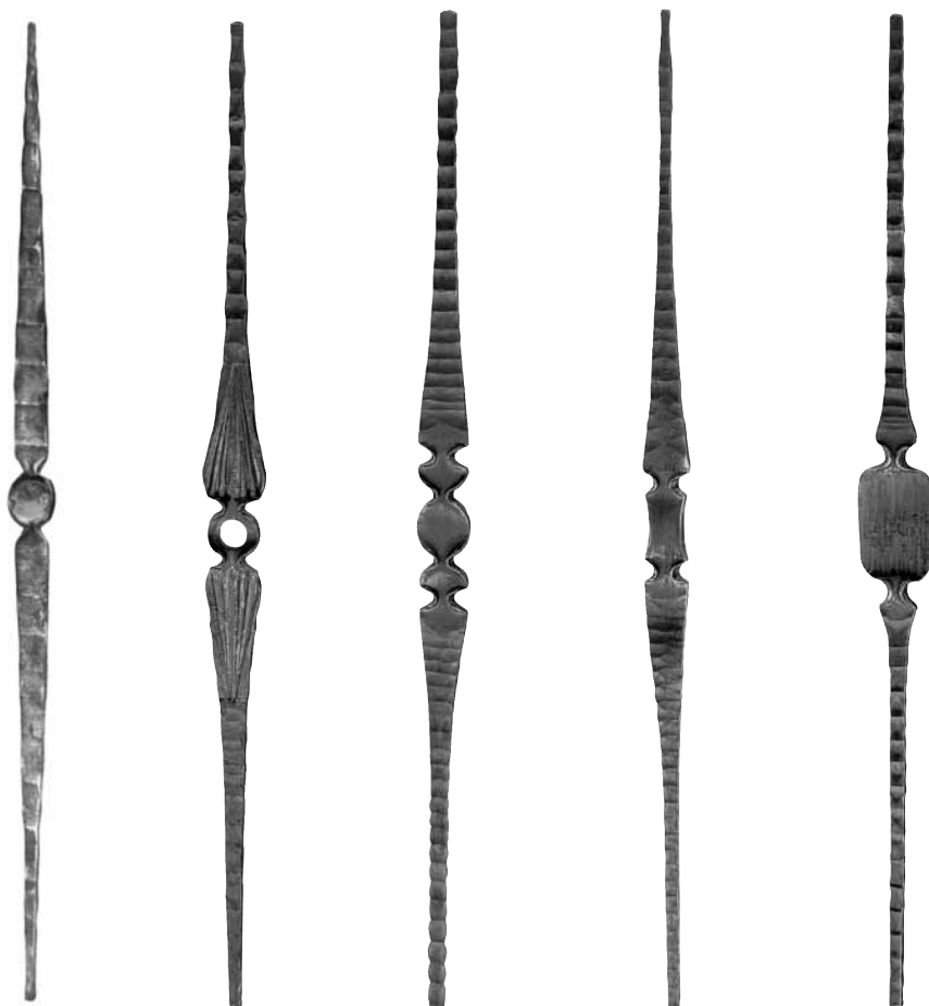
Art. 96/2 Art. 1192/1 Art. 1192/2 Art. 1192/3 Art. 1192/4 Ø 12 x 12 mm Ø 12 x 8 mm Ø 16 x 8 mm Ø 12 x 10 mm Ø 12 x 10 mm H 830 mm H 1000 mm H 1000 mm H 1000 mm H 1000 mm
