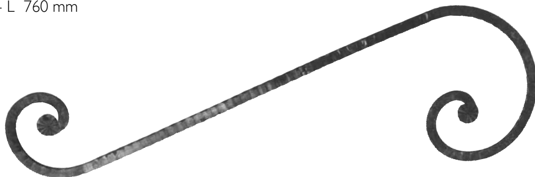
Art. 1281/4 ☒ 16 x 8 mm H 260 mm - L 760 mm
