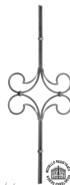
Art. 1053/1 Ø 24 x 12 mm H 1000 mm L 360 mm
