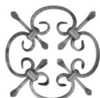
Art. 1015/1 ∅ 8 x 8 mm ∅ 275 mm
