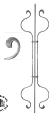
Art. 1075/2 Ø 10 mm H 1000 mm L 245 mm
