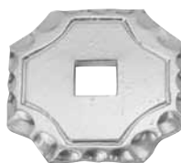
Art. 1426/5 70 x 70 mm foro/hole 12 x 12 mm spess./thick. 4 mm
