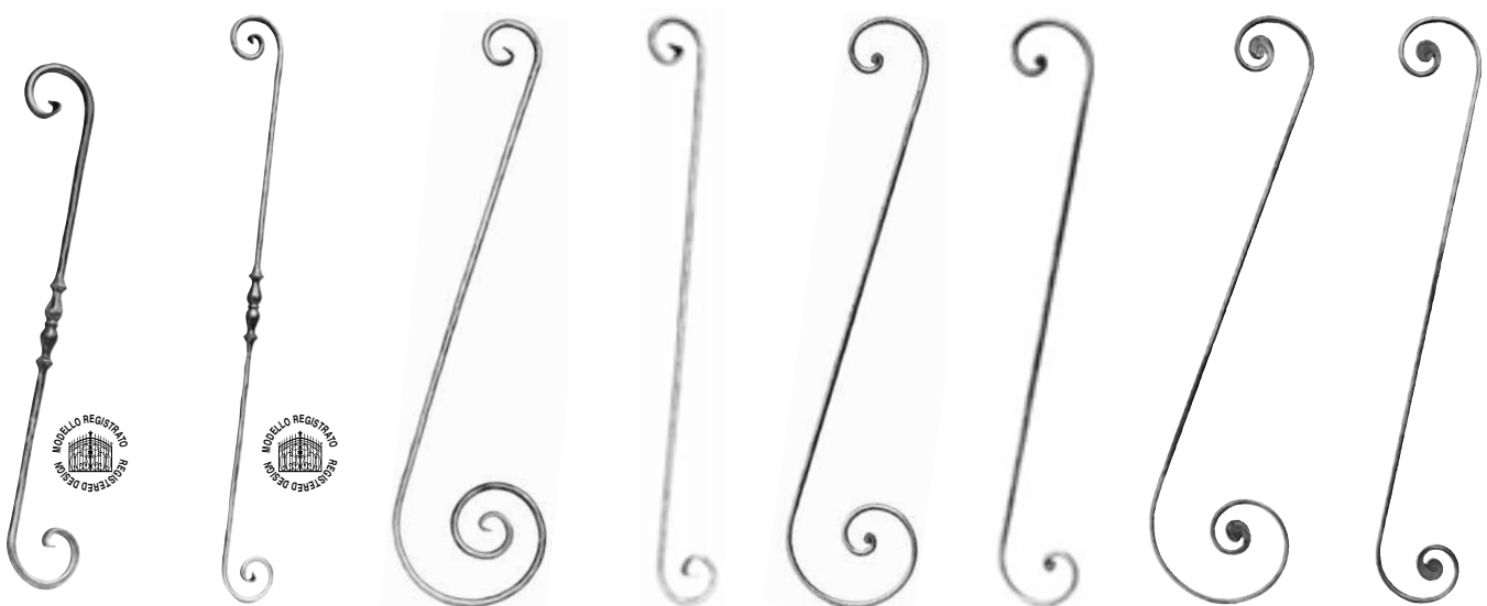
Art. 498/1 Ø 12 mm H 650 mm Forgiati a caldo/Hot forged Art. 498/2 Ø 900 mm H 900 mm Art. 646/1 Ø 12 mm H 900 mm L 250 mm Art. 646/2 Ø 12 mm H 900 L 100 mm Art. 648/4 Ø 10 mm H 900 L 200 mm Art. 648/1 Ø 10 mm H 900 L 120 mm Art. 642/2 Ø 10 mm H 900 mm L 220 mm Art. 642/1 Ø 10 mm H 900 mm L 130 mm
