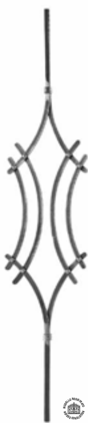
Art. GD21/3 \varnothing 12 x 12 mm H 1000 mm L 200 mm
