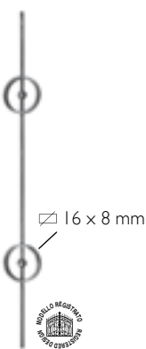
Art. 1082/4 Ø 10 mm H 1000 mm L 100 mm
