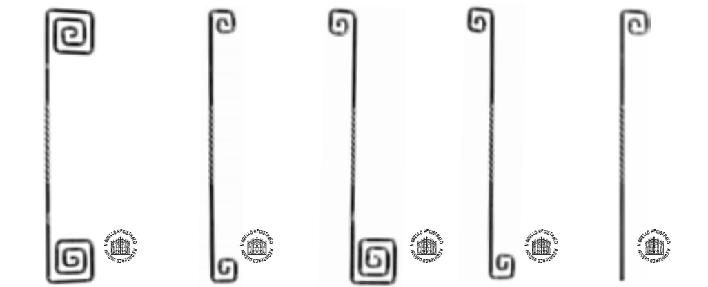
Art. 1147/1 \Phi 12 x 12 mm H 1000 mm L 185 mm Art. 1147/2 \Phi 12 x 12 mm H 1000 mm L 110 mm Art. 1147/3 \Phi 12 x 12 mm H 1000 mm L 280 mm Art. 1147/4 \Phi 12 x 12 mm H 1000 mm L 205 mm Art. 1147/5 \Phi 12 x 12 mm H 1000 mm L 110 mm
