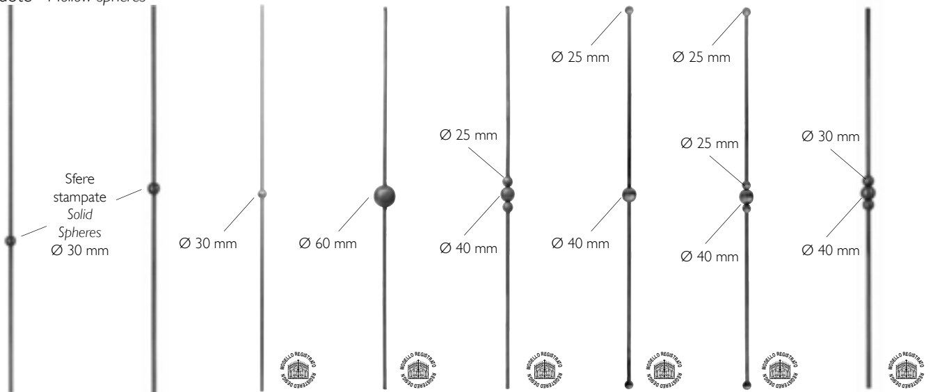
Art. GD247/2 Art. GD247/3 Art. GD92/1 Art. I208/1 Art. I208/2 Art. I208/3 Art. I208/4 Art. GD48/2 Ø 12 mm Ø 12 mm Ø 12 mm Ø 12 mm Ø 12 mm Ø 12 mm Ø 12 mm Ø 12 mm H 1000 mm H 1000 mm H 1000 mm H 1000 mm H 1000 mm H 1200 mm H 1000 mm H 1000 mm
