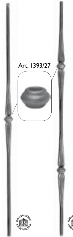
Art. 1177/5 Art. 1177/6 Ø 12 mm Ø 12 mm H 1000 mm H 1000 mm
