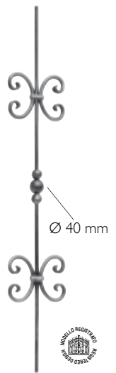
Art. 1064/2 Ø 12 mm H 1000 mm L 175 mm
